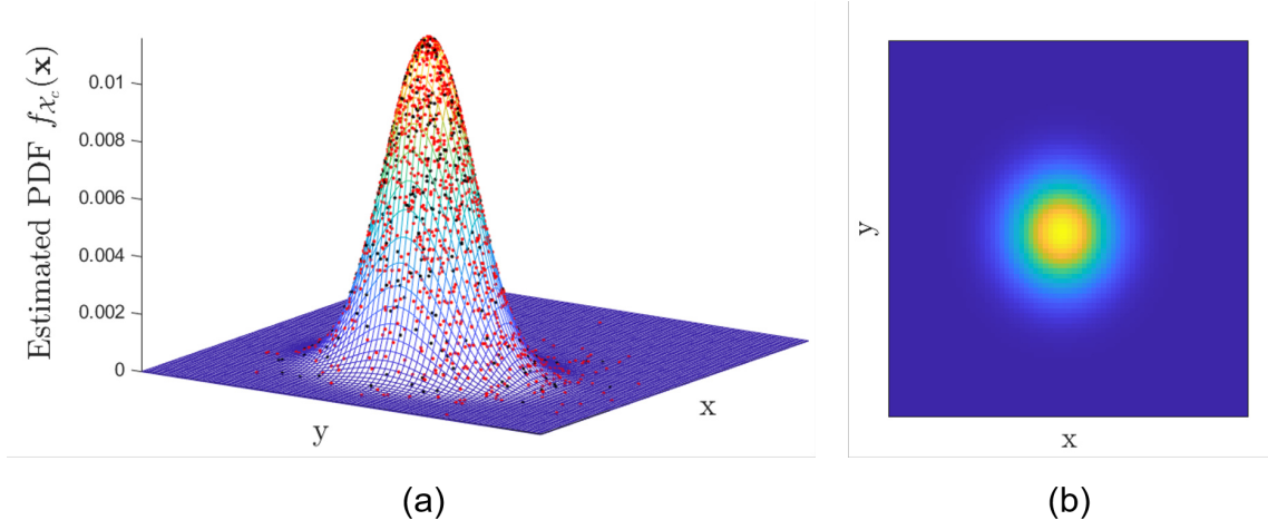
Figure 2. The Maximum Likelihood Estimated pdf f_{\mathcal{X}_c}(\mathbf{x}_c) of the Random Variable \mathcal{X}_c resulting from a small sample of 128 black dotted ground-truth eye centers of the face database BioID and the remaining red dotted ground-truth centers superimposed onto the estimated pdf (a). Top view of the f_{\mathcal{X}_c}(\mathbf{x}_c) uncovering its isotropic nature (b)
