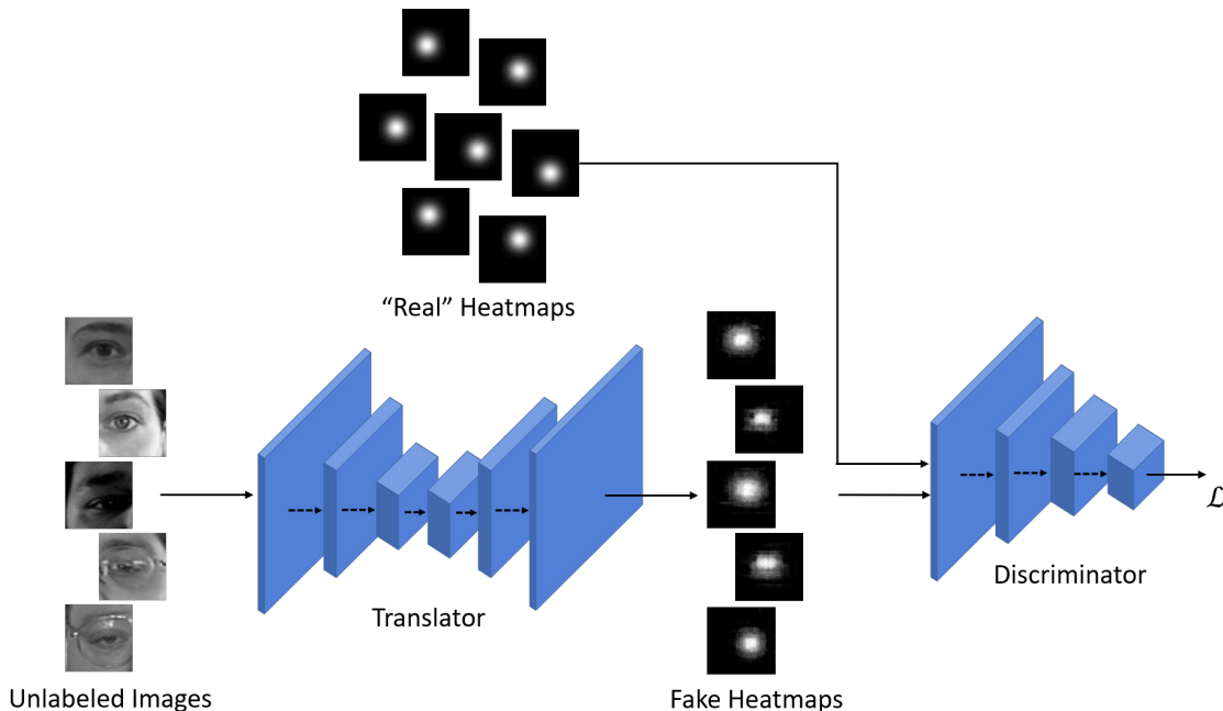
Figure 3. PupilTAN Deep Architecture
