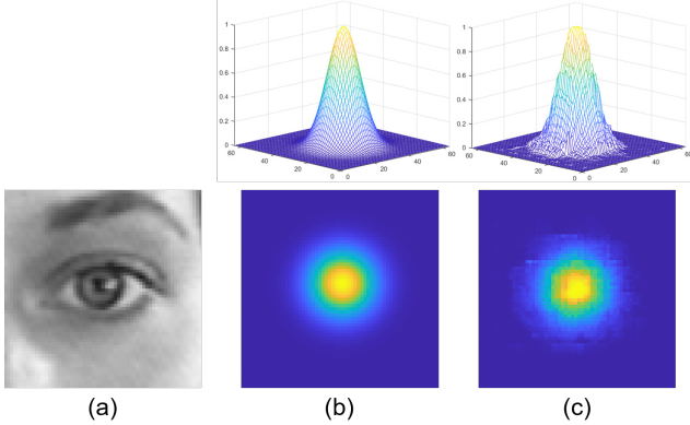
Figure 1. The eye’s region around its center (a), its idealization modelled by a heatmap with center at the pixel where the real eye’s center is located and std equal to the radius of the circle that covers the iris area (b), and the fake heatmap achieved by PupilTAN (c)
